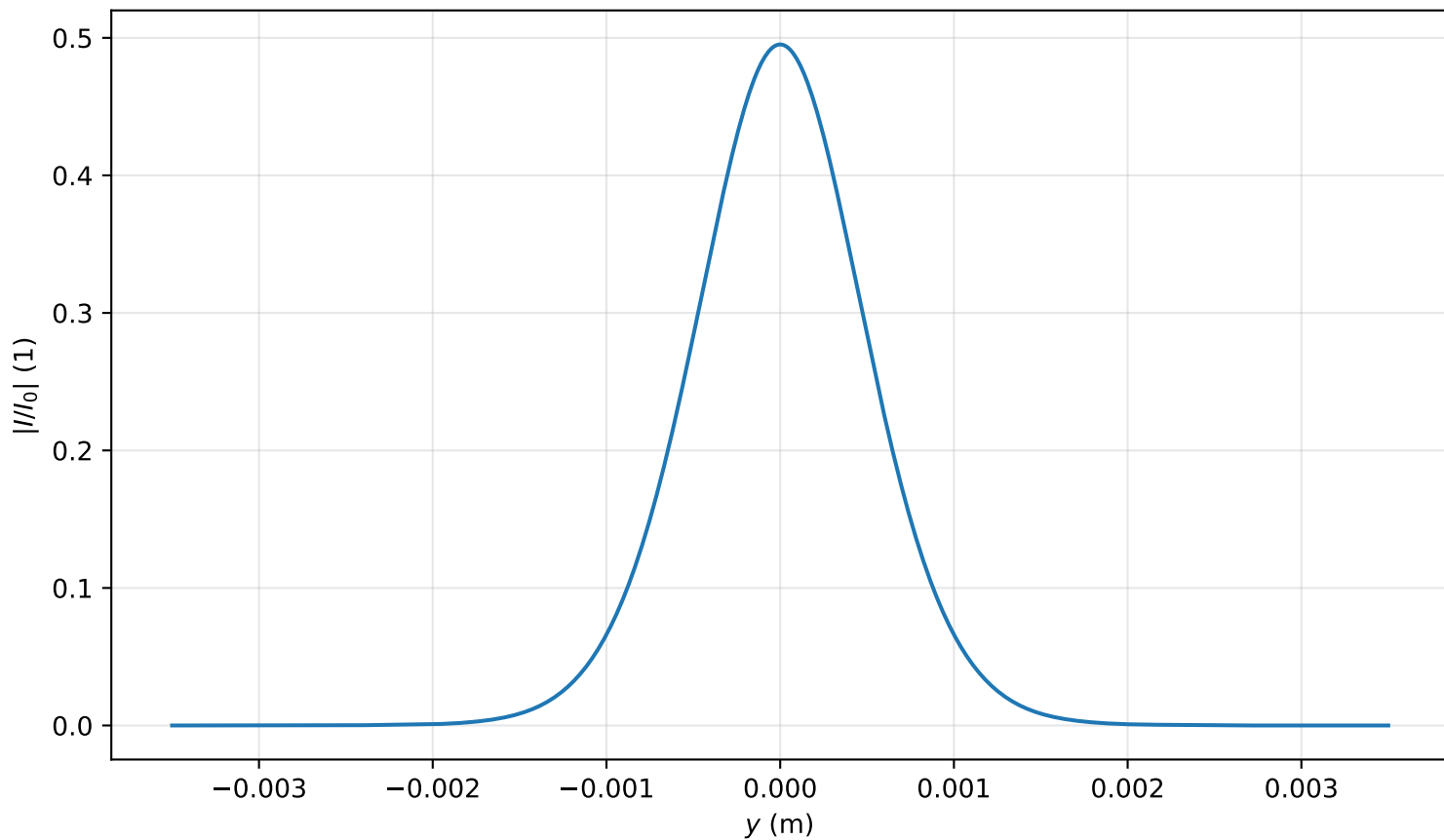
Intensity profile I(x=0, y, z=2.946)/I_0 , P_{in}=0.4P_{cr} , artificial time
